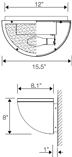
WMUL = wall mount uplight
