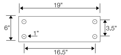
Bollard base detail
