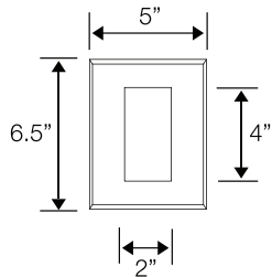
Wall mount bracket detail
